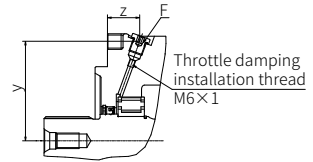
V32G flushsectional view
