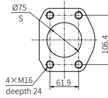
Suction port S
