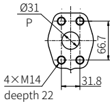
Pressure port P
