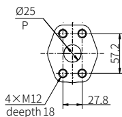
Pressure port P
