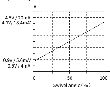
Output voltage/current
