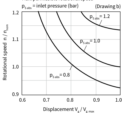
▼ Max. permissible rotational speed
