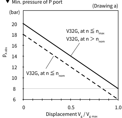
▼ Min. pressure of P port
