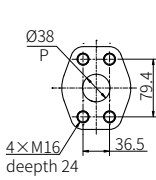
Pressure port P
