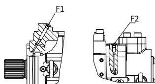
Variable displacement pump without flushing function
