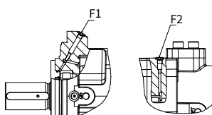
Quantitative pump without flushing function
