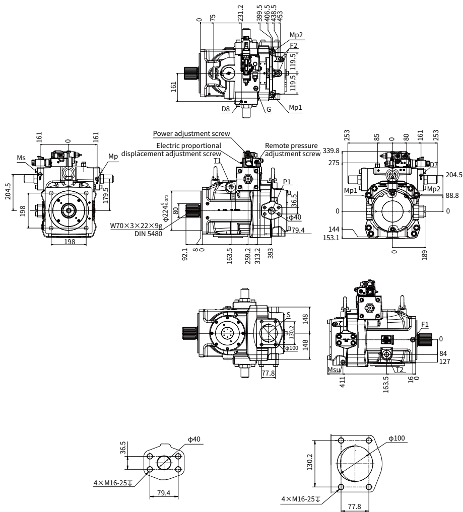
Pressure port P1, P2
