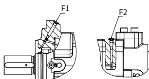
Quantitative pump with flushing function
