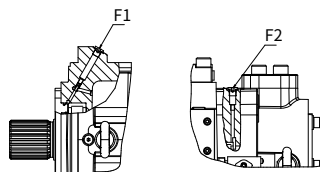
Variable displacement pump with flushing function
